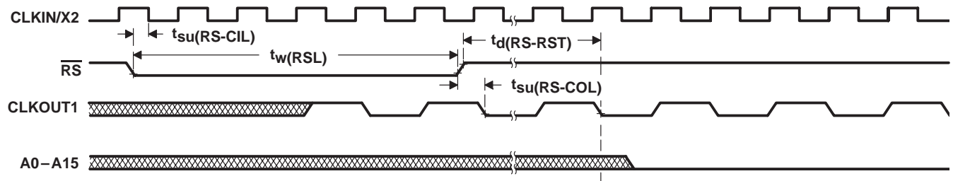
Figure 13. Reset Timing
